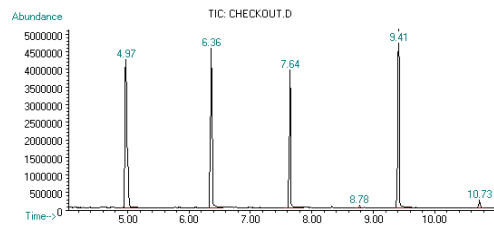
Gas chromatogram
