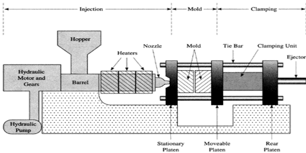
Figure 1 Injection molding machine showing three major functional units (injection, mold, and clamping) along with major components of each unit.
