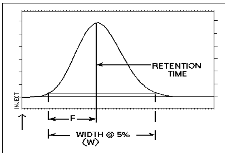
Figure 3: 2.4 USP Tailing
