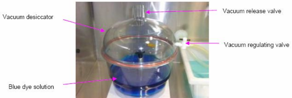
Figure: 2 Vacuum Leak Test Apparatus
