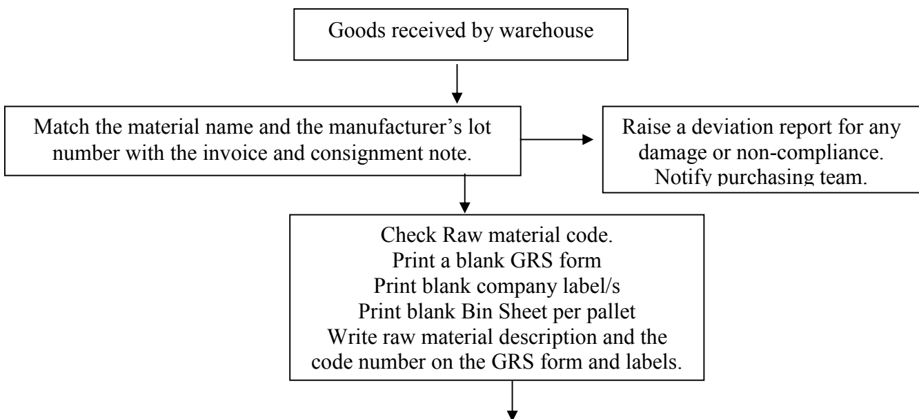
Figure 3: Branching Flowchart
